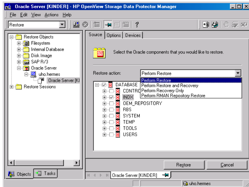
Figure 1-23 Source Pane
