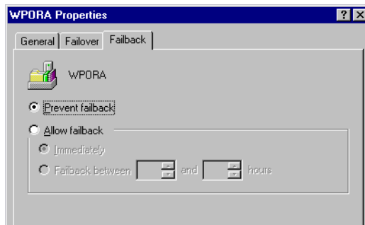
Figure 1-21 Checking Properties
