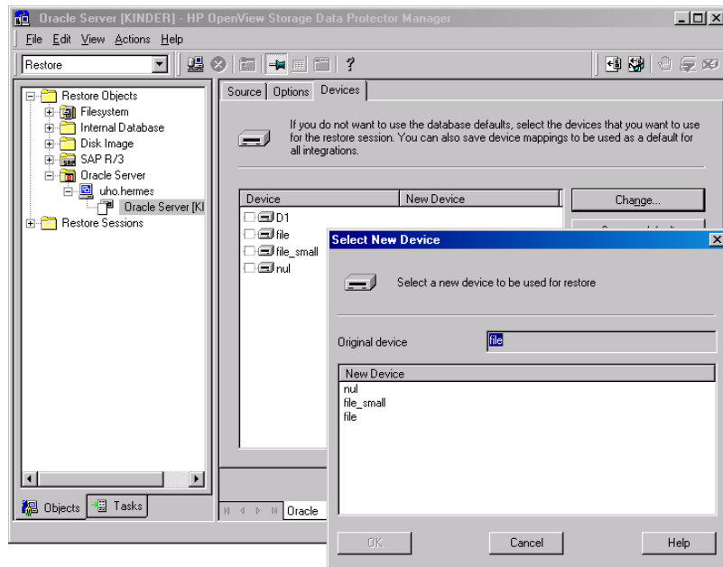
Figure 1-25 Devices Pane
