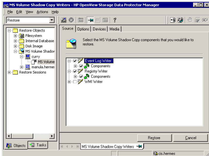
Figure 5-10 Restore Objects
