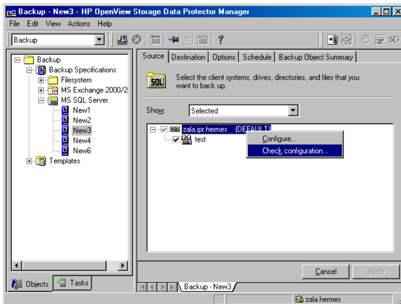
Figure 3-4 Checking Configuration
