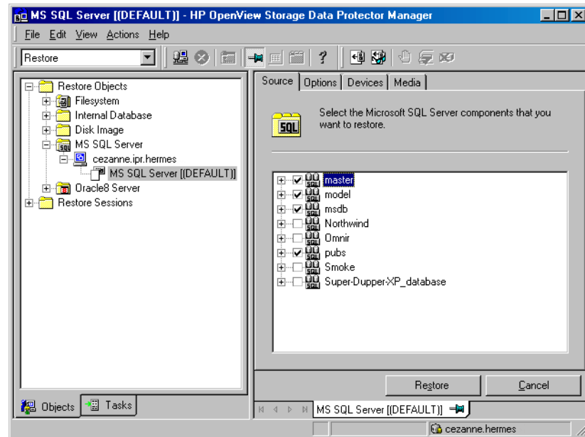
Figure 3-16 Restore Objects
