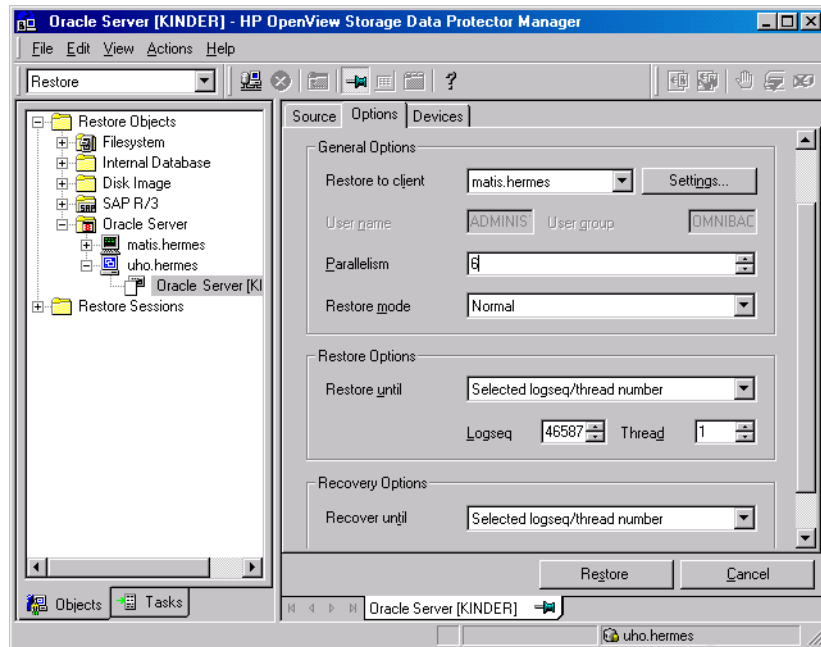
Figure 1-24 Options Pane
