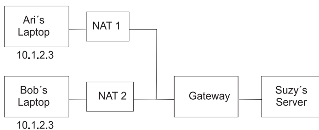
Figure 13. Tunnel Mode Conflict
