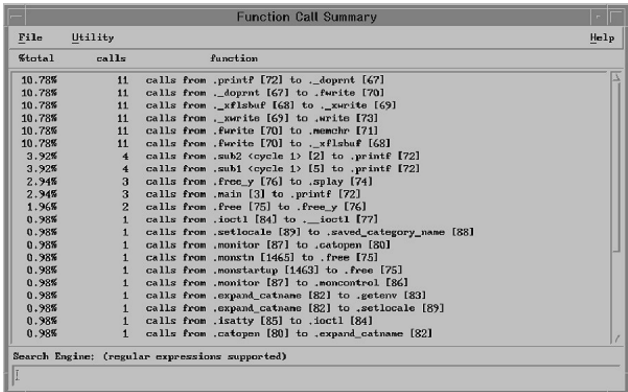
Figure 23. The Function Call Summary report. The screen capture below shows an example of the Function Call Summary Report window. There is a menu bar at the top with the following options: File, Utility, and Help. There is a list of all the functions in your application that call other functions and they appear as caller-callee pairs (call arcs, in the function call tree), and are sorted by the number of calls in descending order.
