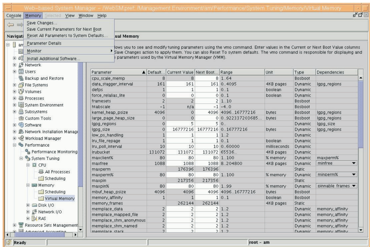
Figure 37. Tables Menus window
