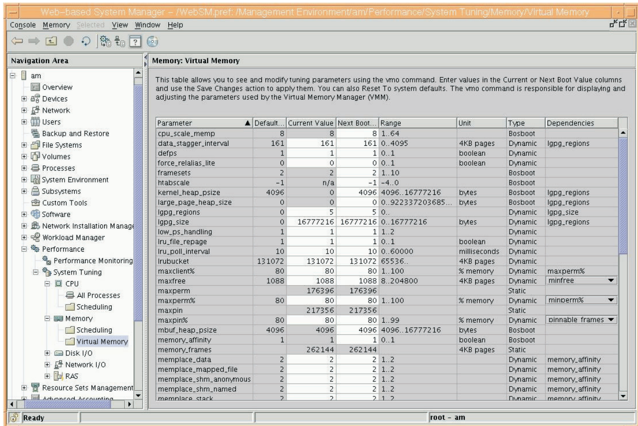
Figure 36. Memory VMM window
