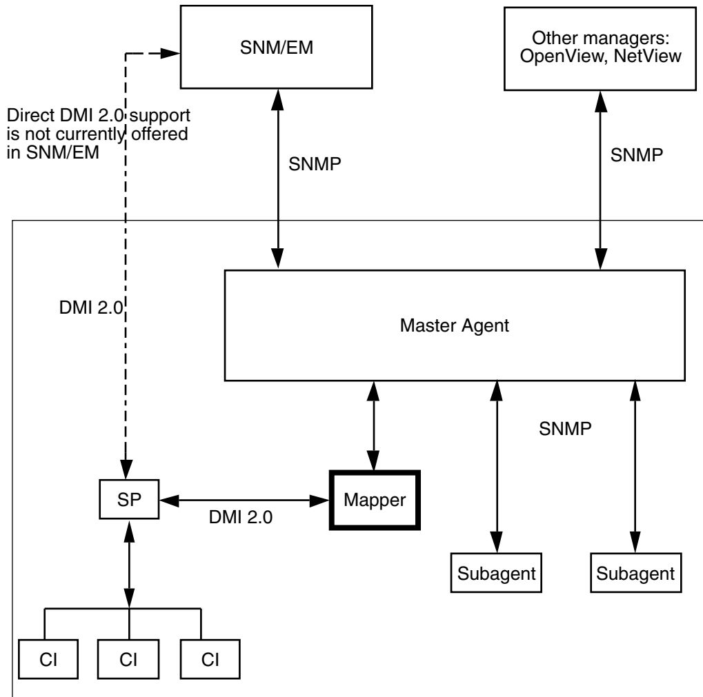
FIGURE 6-1 snmpXdmi.d Overview
