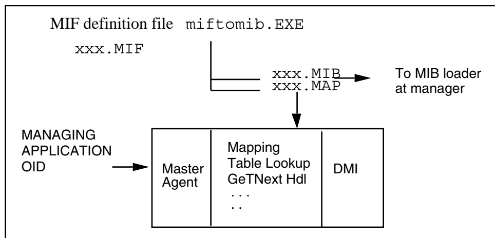
FIGURE 6-2 MIF-to-MIB Mapping
