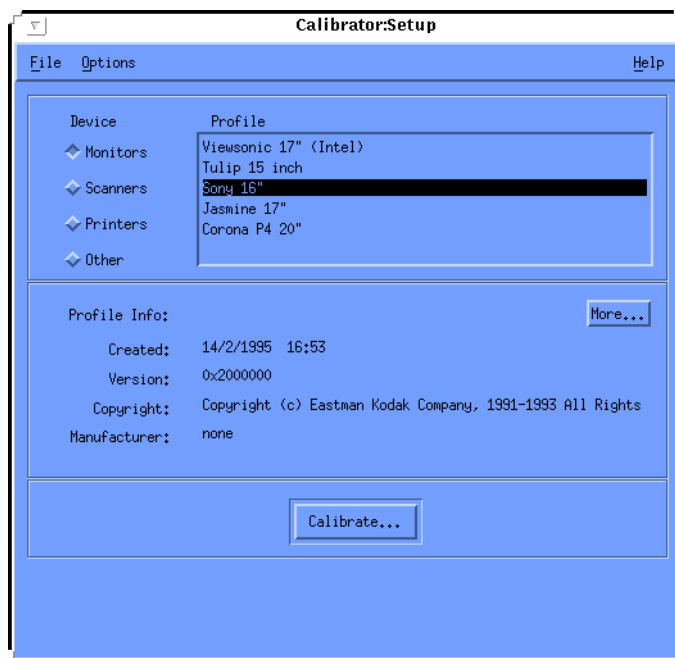
FIGURE 2-1 Calibrator Tool Setup Window
