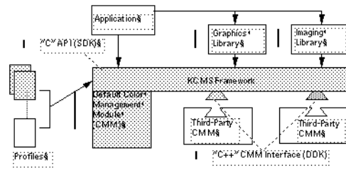
FIGURE 1-1 KCMS Architecture
