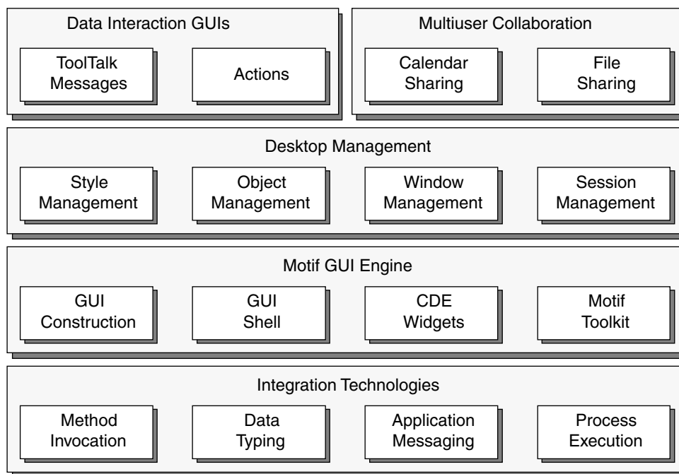
FIGURE 1-1 Conceptual overview of Common Desktop Environment
