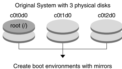
FIGURE 35-1 Detaching and Upgrading One Side of a RAID-1 Volume (Mirror) (continued)
