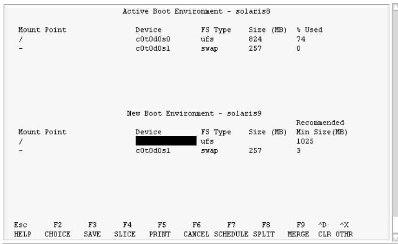
FIGURE 35-4 Solaris Live Upgrade Configuration Menu
