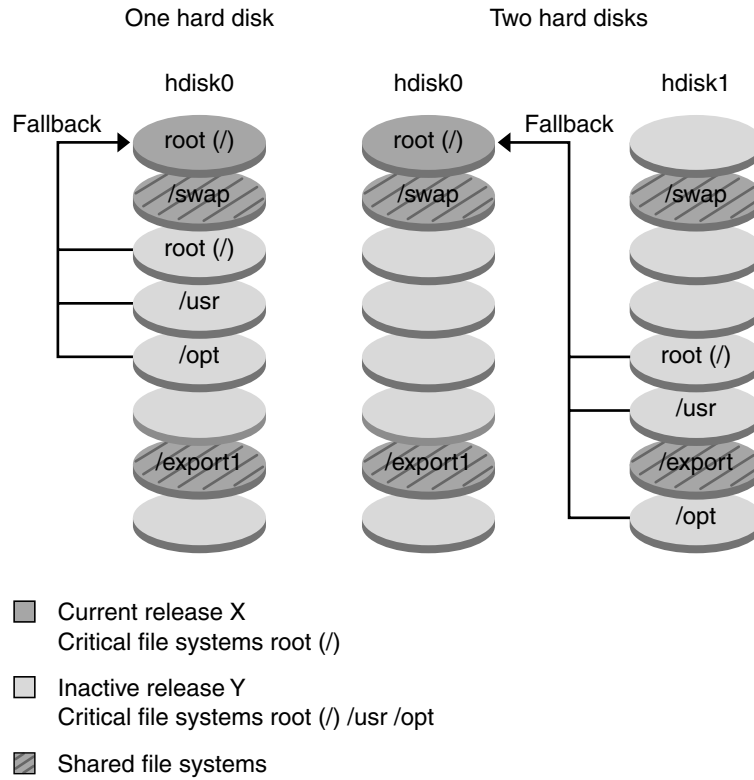
FIGURE 30-9 Fallback to the Original Boot Environment
