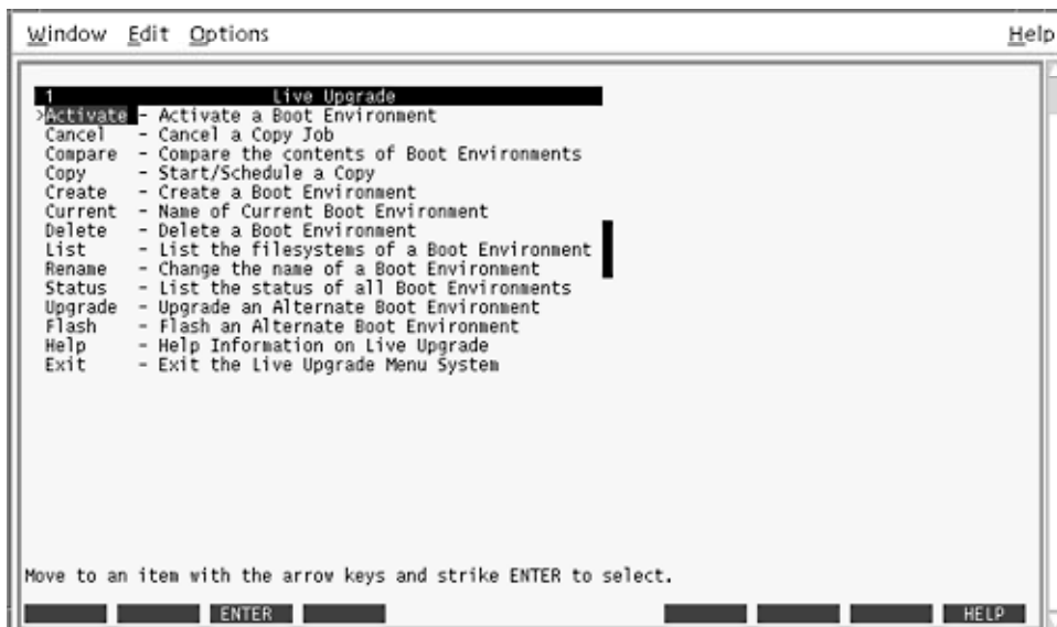
FIGURE 35-3 Solaris Live Upgrade Main Menu
