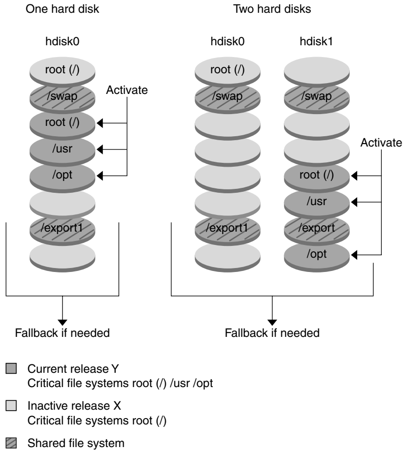
FIGURE 30-8 Activating an Inactive Boot Environment
