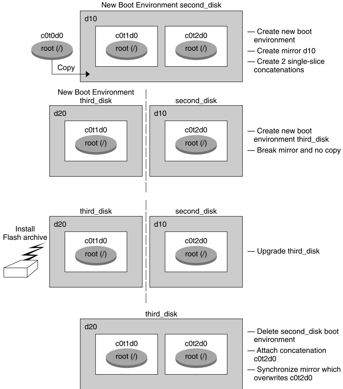
FIGURE 35-2 Detaching and Upgrading One Side of a RAID-1 Volume (Mirror) (continued)
