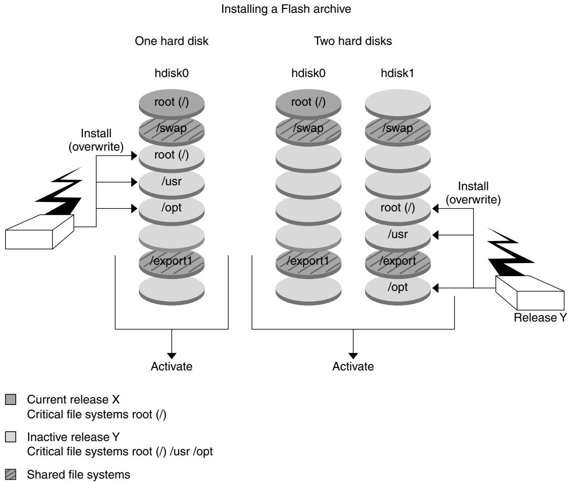
FIGURE 30–7 Installing a Solaris Flash Archive
