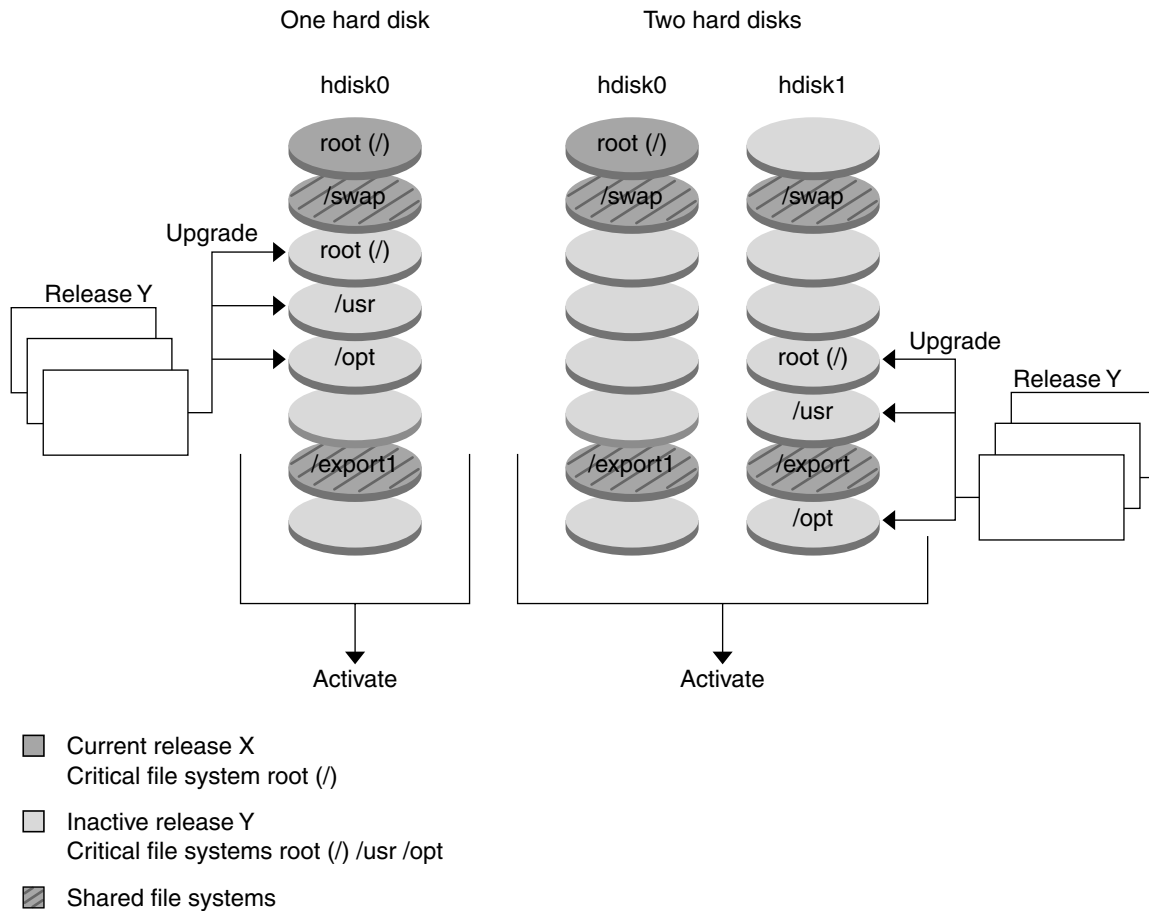
FIGURE 30-6 Upgrading an Inactive Boot Environment
