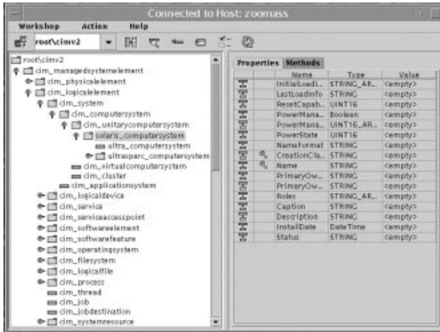
Figure 2-1 Class Inheritance Tree in CIM WorkShop Window
