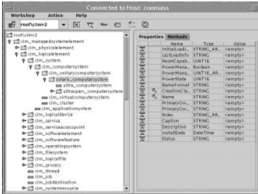
Figure 2-2 The CIM WorkShop Window
