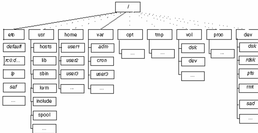
Figure 9-1 Solaris 7 Default File Systems and Directory Hierarchy
