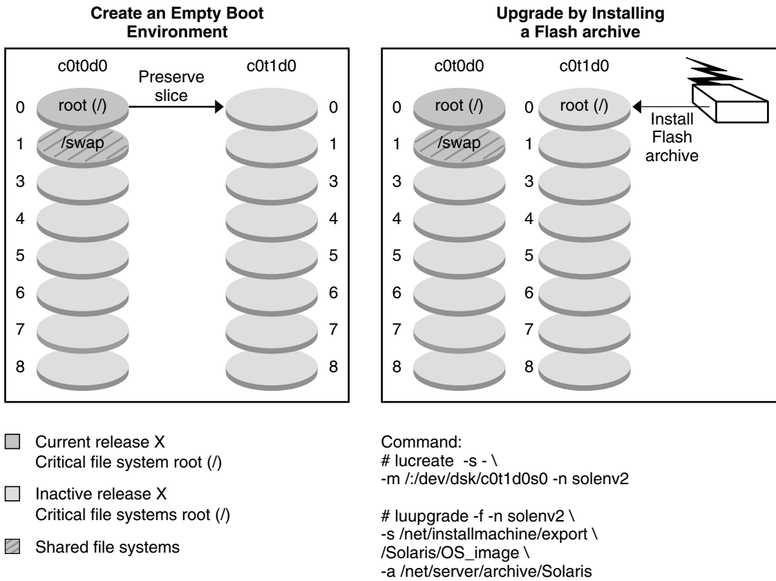
FIGURE 6-9 Installing a Solaris Flash Archive on Two Disks
