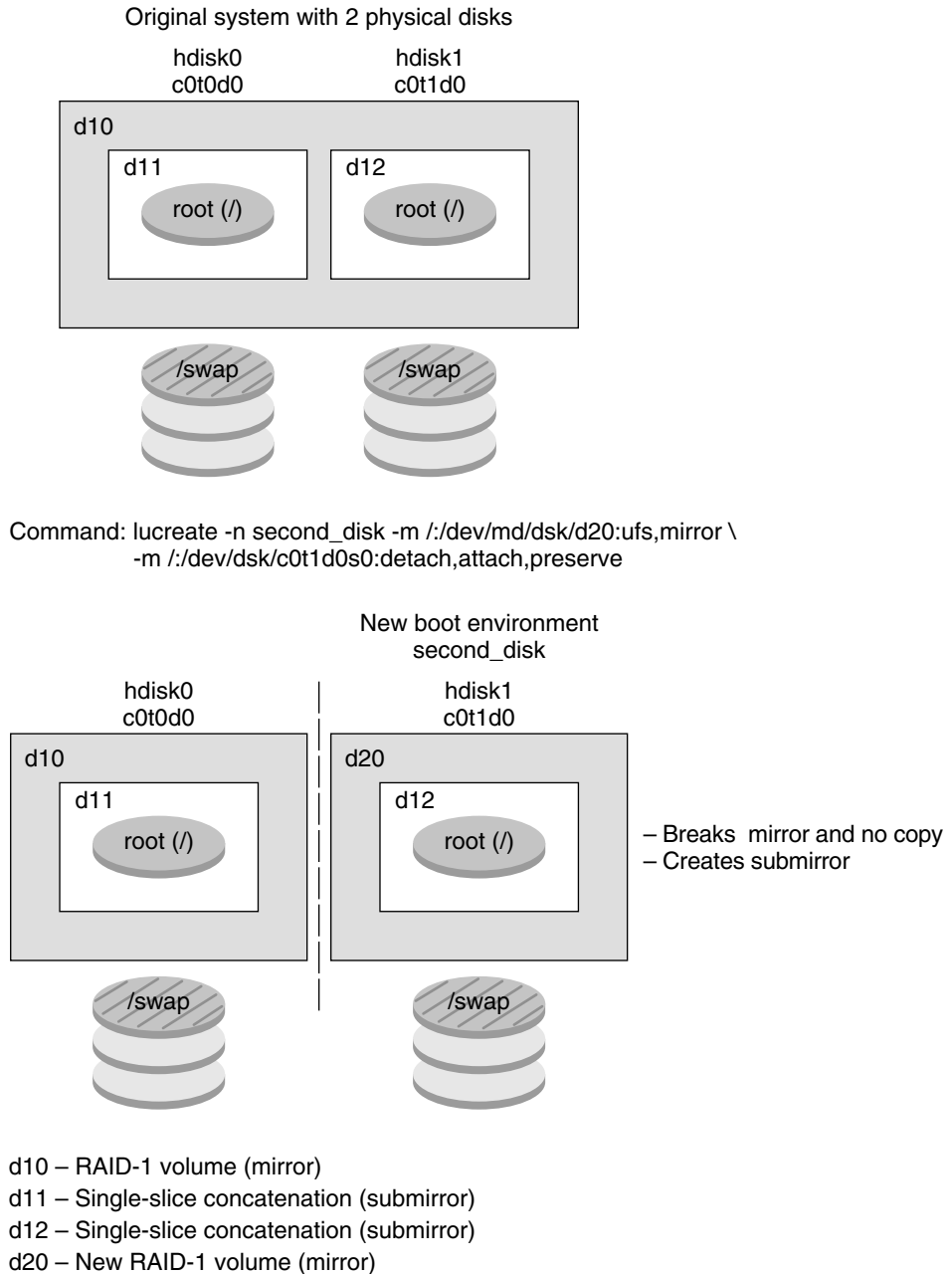
FIGURE 6-6 Create a Boot Environment and Use the Existing Submirror
