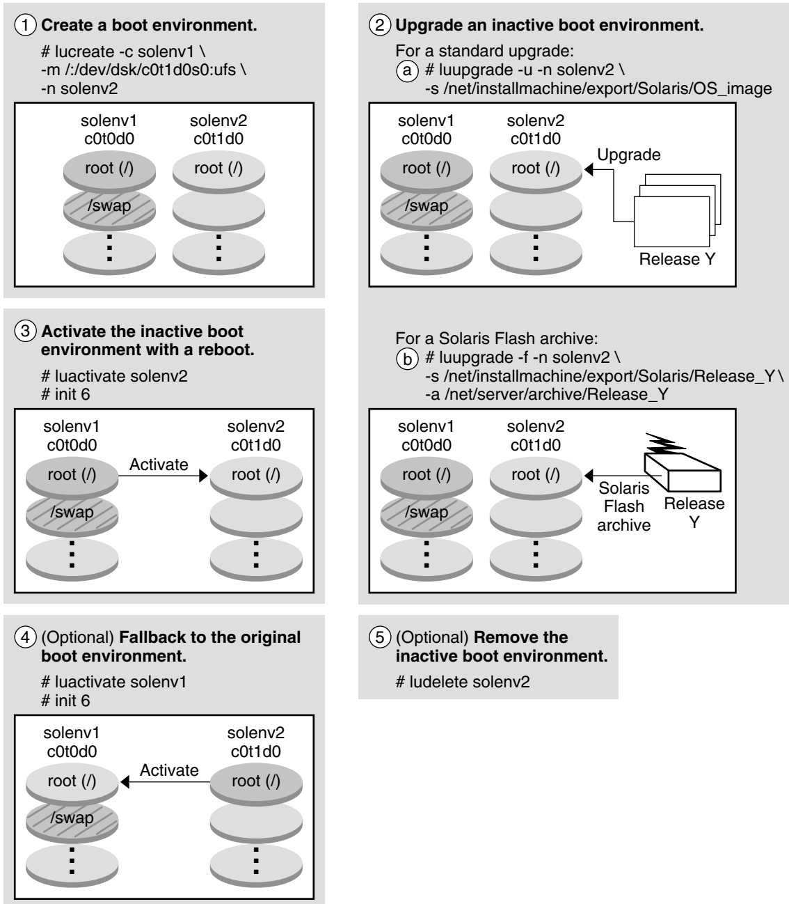
FIGURE 6-1 Solaris Live Upgrade Process
