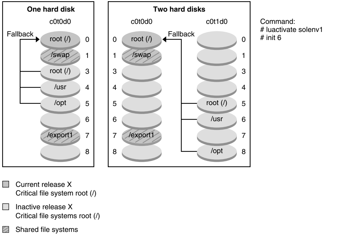
FIGURE 6-11 Fallback to the Original Boot Environment
