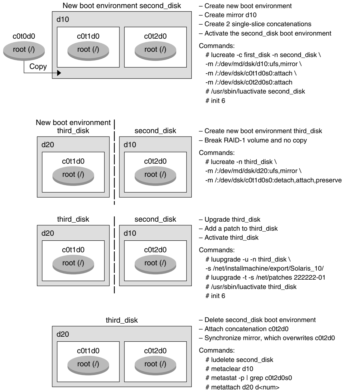
FIGURE 12-2 Detaching and Upgrading One Side of a RAID-1 Volume (Mirror) (continued)
