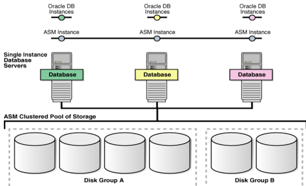
Figure 1–3 ASM Cluster with Single-Instance Oracle Databases
