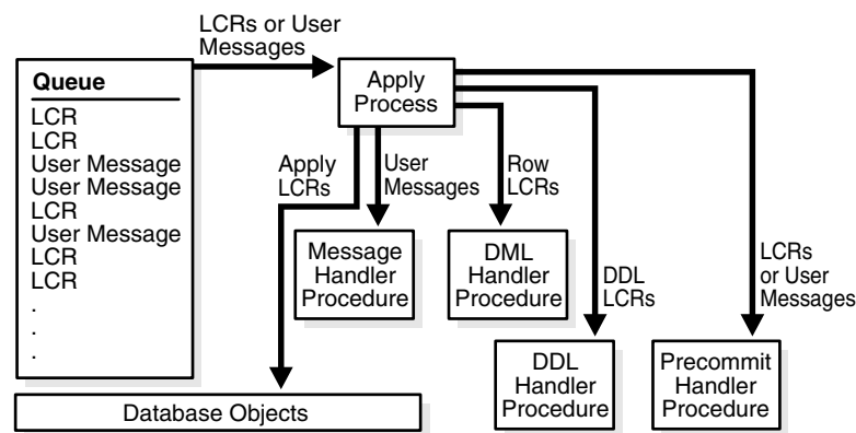
Figure 1-7 Apply Process
