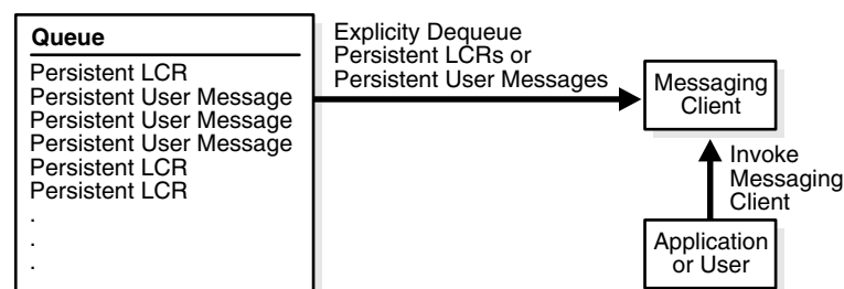
Figure 1-8 Messaging Client
