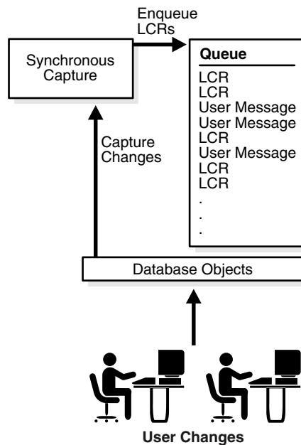
Figure 1–3 Synchronous Capture
