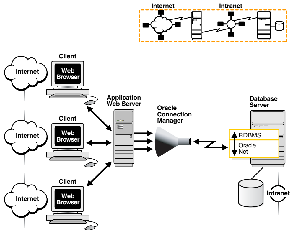
Figure 1–11 Session Multiplexing
