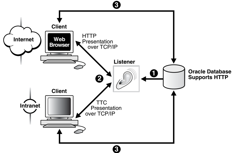
Figure 5–7 Listener Architecture
