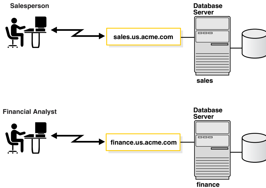
Figure 3–3 One Instance for Each Database
