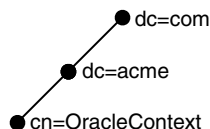
Figure 8-2 Oracle Context
