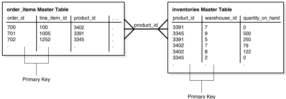
Figure 3-5 Row Subsetting with Many to Many Subqueries
