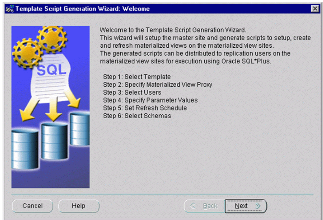
Figure 7–10 Opening Screen of the Template Script Generation Wizard
