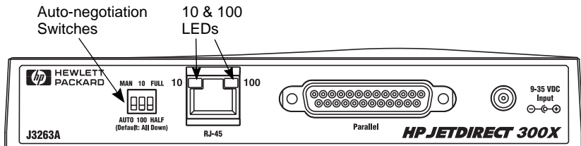
Figure 1.3 Back of HP JetDirect 300X Print Server. (For the HP JetDirect 500X, the LEDs are also located next to the RJ-45 port.)
