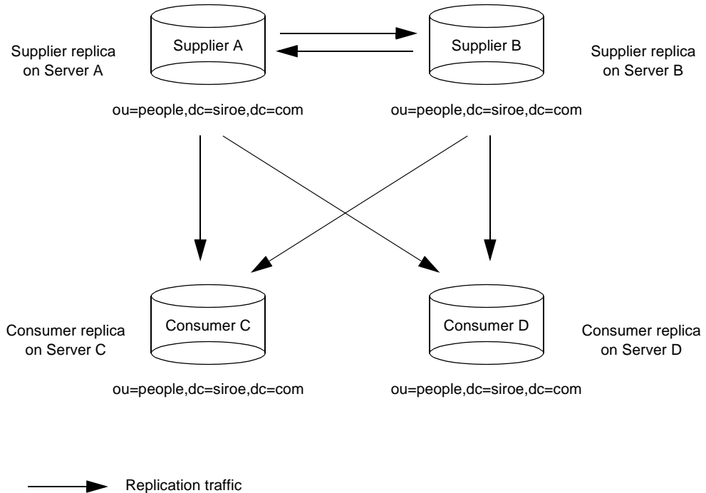
Figure 8-2 Multi-Master Replication
