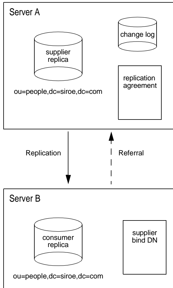
Figure 8-1 Single-Master Replication
