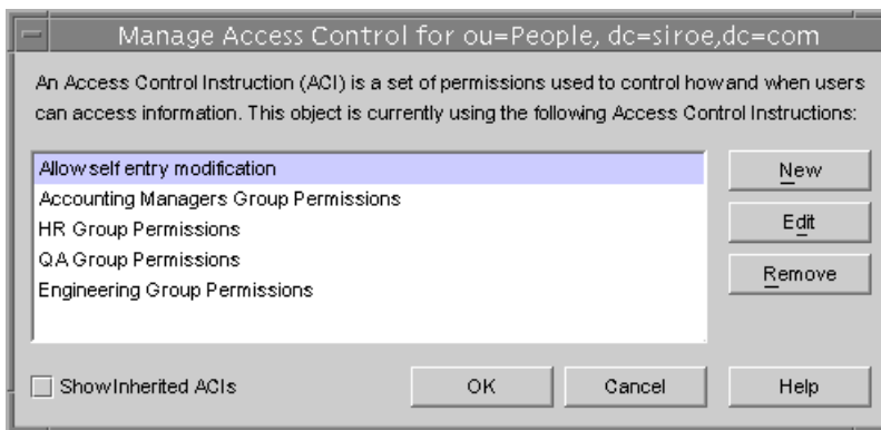
Figure 6-2 The Access Control Management Dialog
