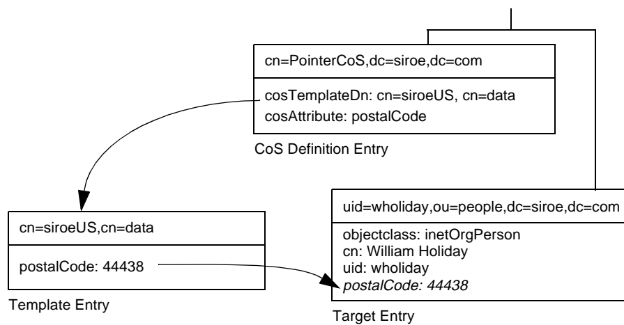
Figure 5-1 Example of a Pointer CoS Definition and Template
