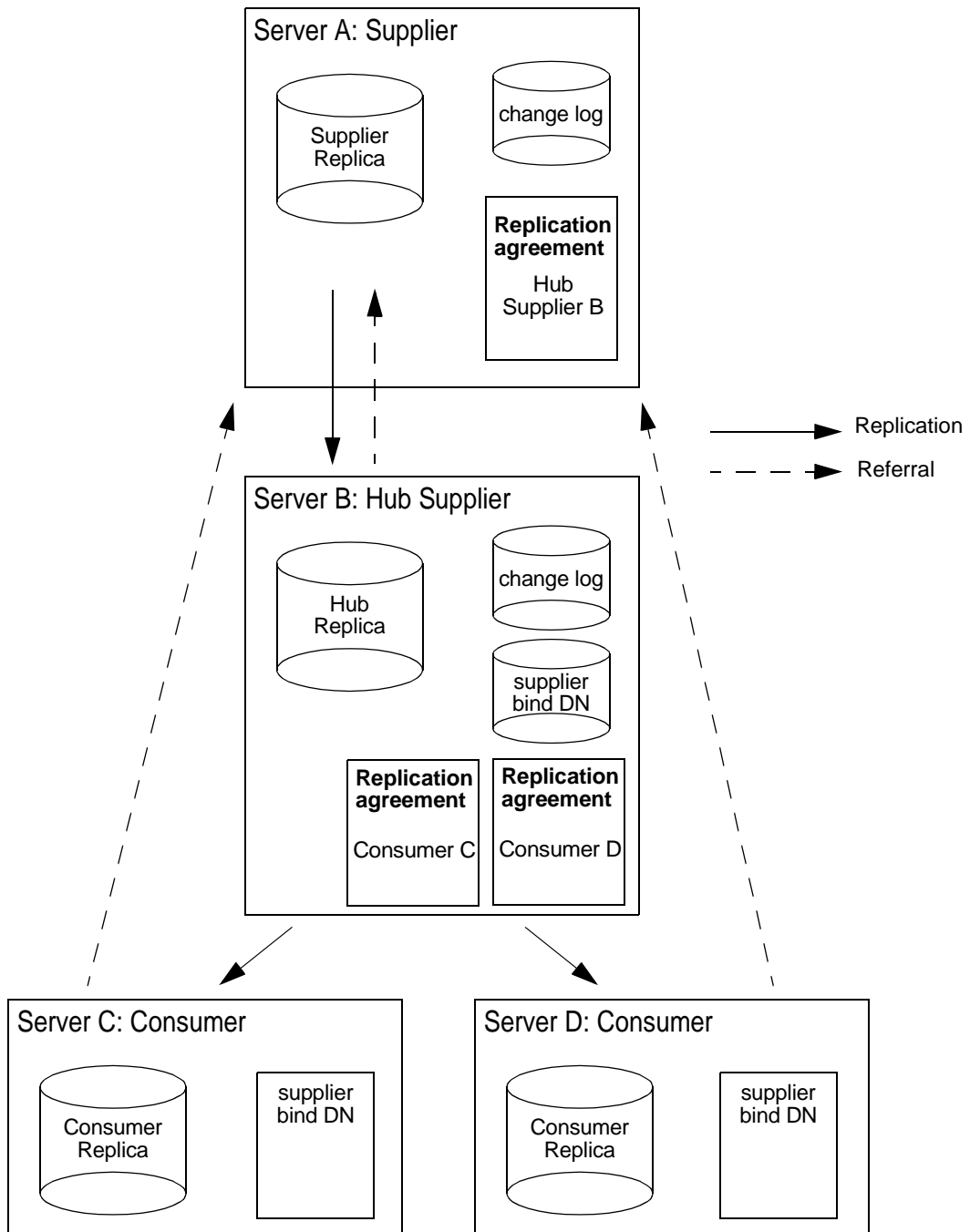
Figure 8-4 Cascading Replication
