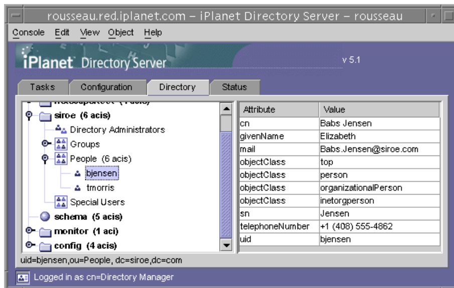
Figure 1-4 Directory Tab of the Directory Server Console
