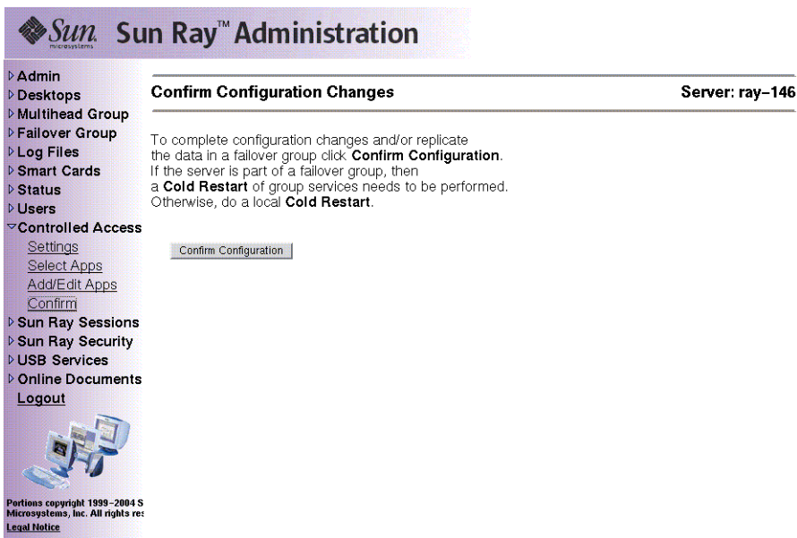
FIGURE 3-37 Confirmation Window
