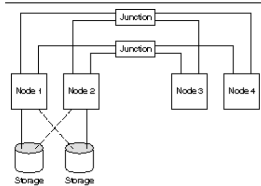
FIGURE 2-4 Pair+N Topology
