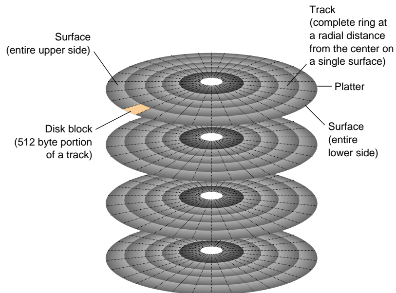
Figure 1-2 Physical Disk Structure
